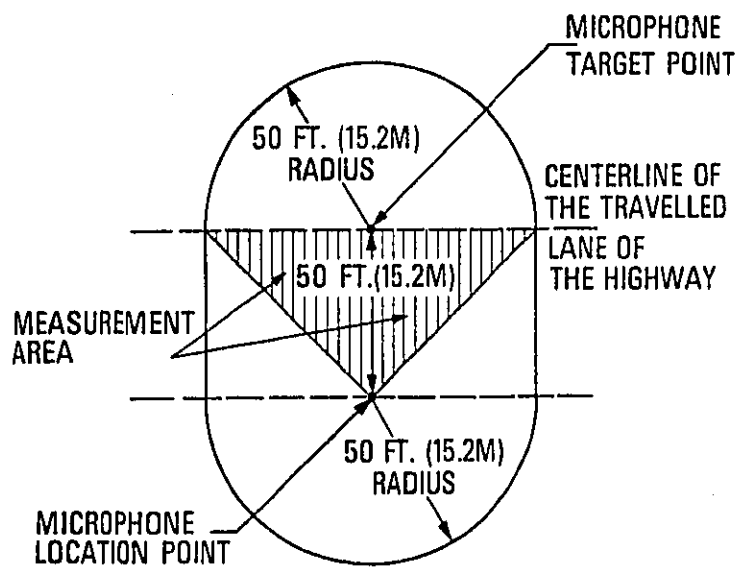
Figure 1 STANDARD TEST SITE; HIGHWAY OPERATIONS
