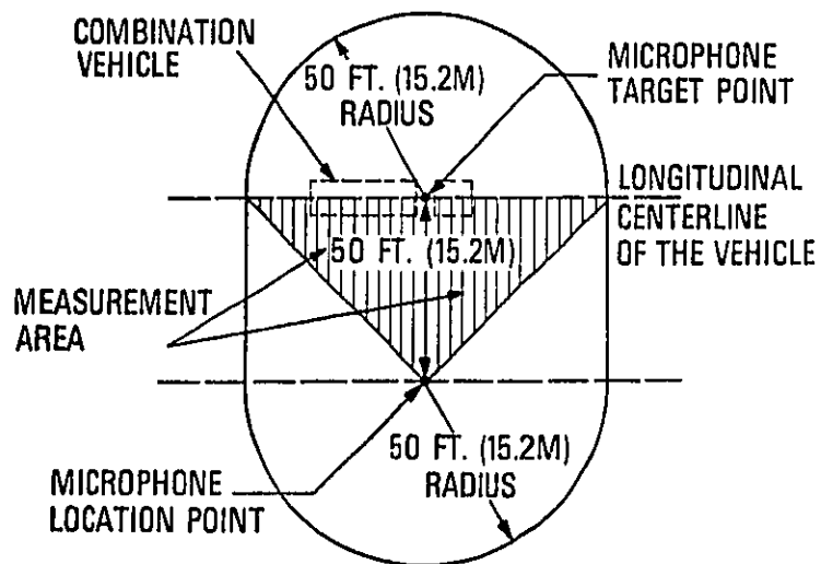
Figure 2 STANDARD TEST SITE; STATIONARY TEST
